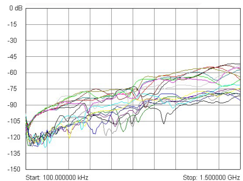
40-755 typical channel to common isolation plot
