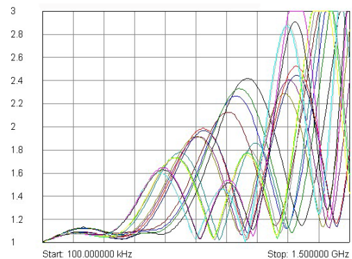
40-755 typical VSWR plot
