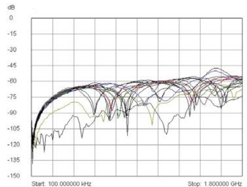
40-755 typical bank to bank crosstalk plot
