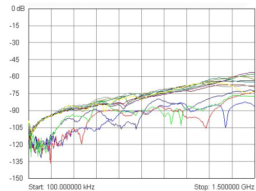
40-755 typical bank to bank crosstalk plot
