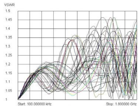
40-755 typical VSWR plot
