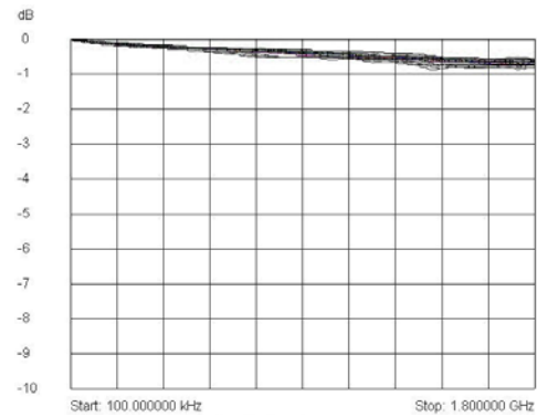
40-755 typical insertion loss plot
