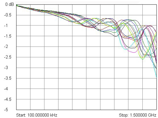
40-755 typical insertion loss plot
