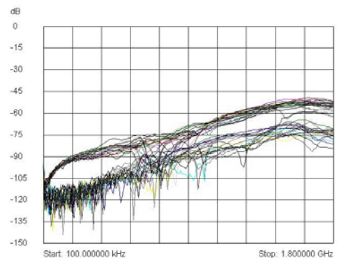
40-755 typical channel to common isolation plot
